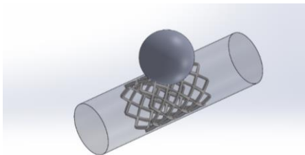
Fig. 1: Placement of Regular Stent in Aneurysm
