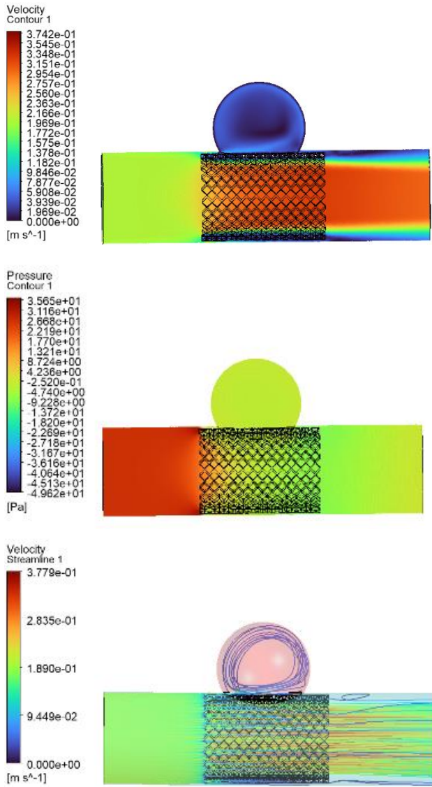
Fig. 6: Velocity Contour, Pressure Contour and Velocity Streamline with Flow Diverter Stent using Non-Newtonian Fluid
