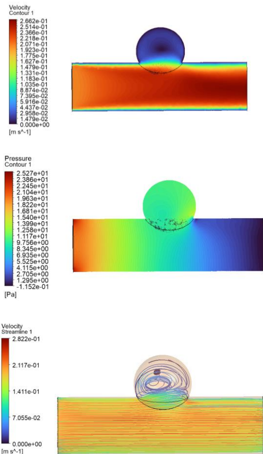
Fig. 3: Velocity Contour, Pressure Contour and Velocity Streamline without stent
