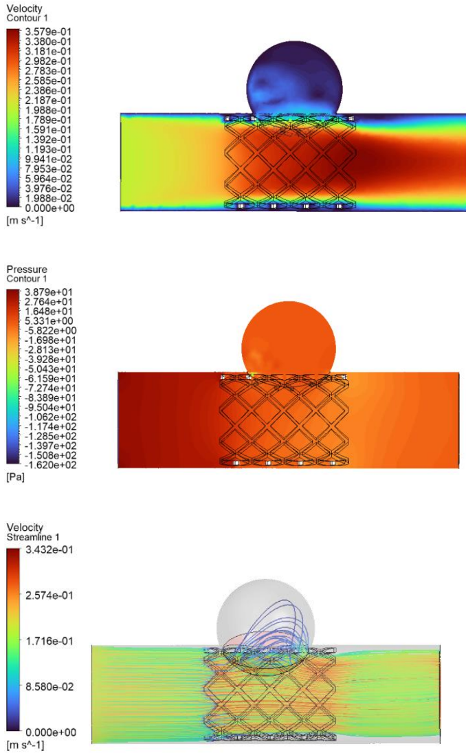
Fig. 4: Velocity Contour, Pressure Contour and Velocity Streamline with Regular Stent
