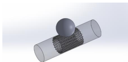
Fig. 2: Placement of Flow Diverter Stent in Aneurysm
