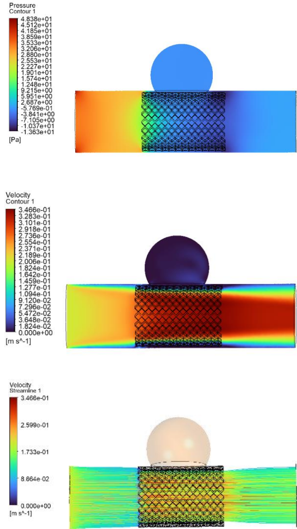
Fig. 5: Velocity Contour, Pressure Contour and Velocity Streamline with Flow Diverter Stent
