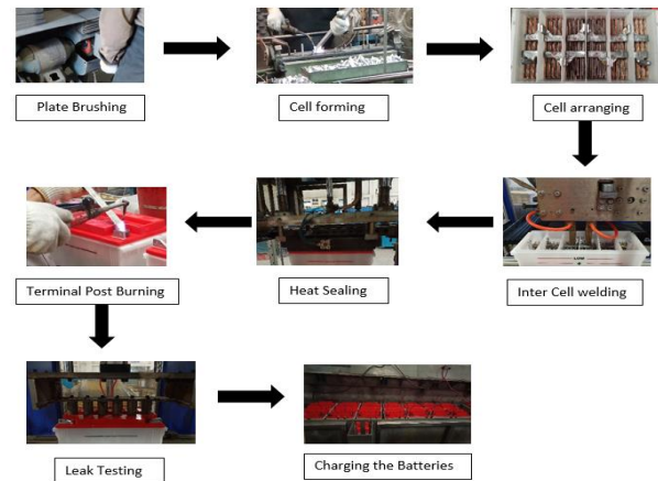
Fig.3 Diagram of experimental process
