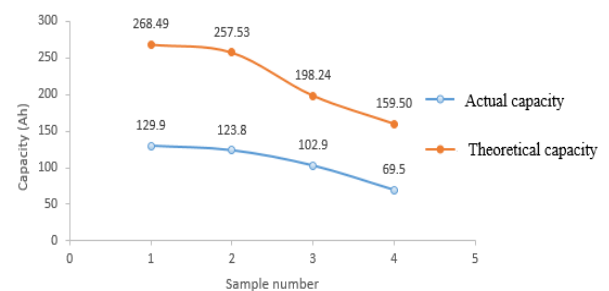
Fig.5 Active mass utilization co-efficient vs sample number graph showing theoretical capacity and actual capacity
