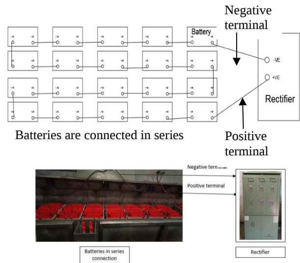
Fig.4 Experimental setup. [7]
