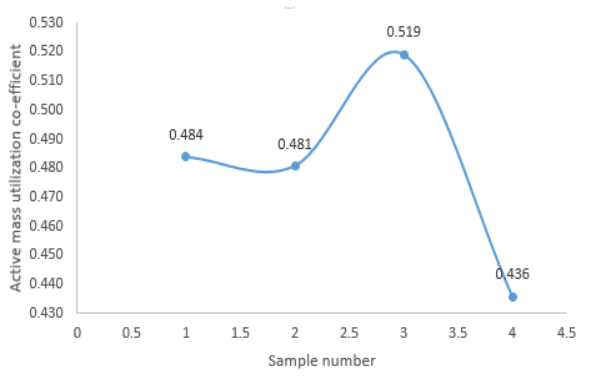
Fig.6 Active mass utilization co-efficient vs sample number graph
