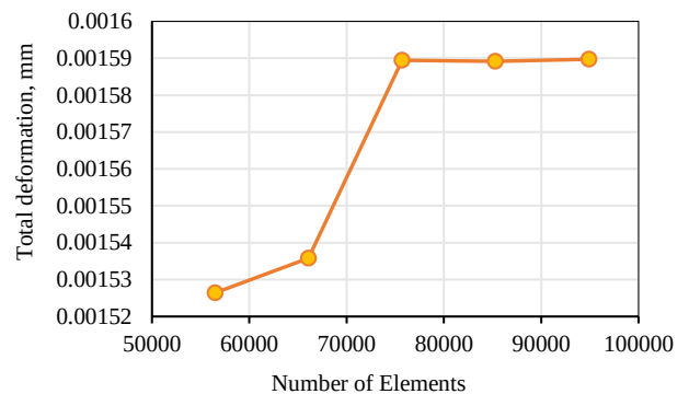
Fig.7 Mesh dependency result for structural analysis
