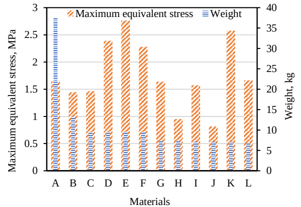
Fig.11 Maximum equivalent stress for various materials
