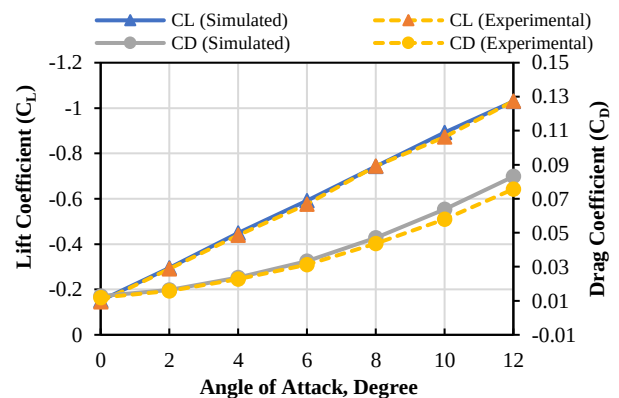
Fig.3 Drag and lift coefficient for simulation and experiment
