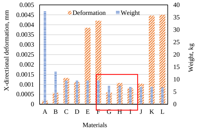
Fig.8 X-directional deformation and weight for various materials (X and Y inside the parentheses indicate the fiber direction of unidirectional composite)
