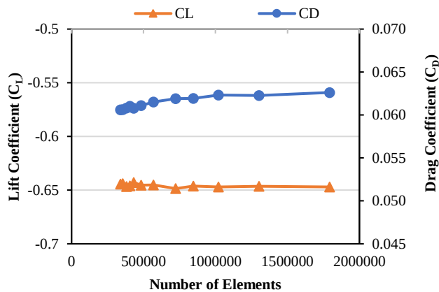
Fig.5 Mesh dependency of lift and drag coefficient for the main design
