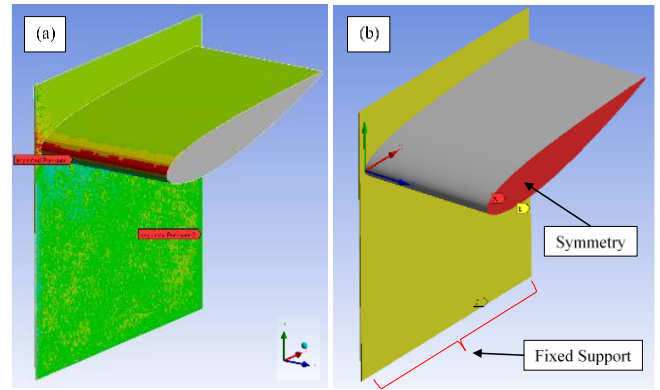
Fig.6 (a) Pressure load on the wing and the endplates and (b) Boundary conditions (the movement of the endplates along the z-axis is restricted).
