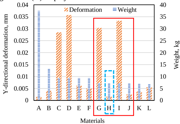
Fig.9 Y-directional deformation and weight for various materials
