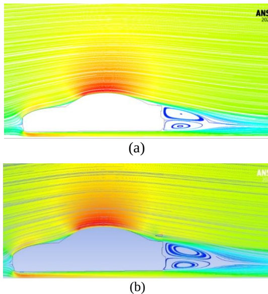
Fig.10 Velocity Stream line (a) without spoiler (b) with spoiler
