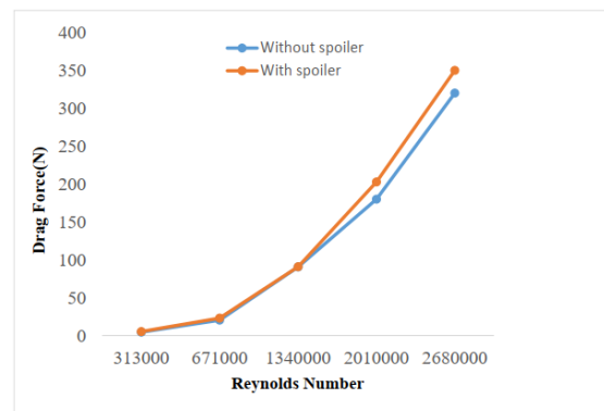
Fig.13 Drag force variation with Reynolds number
