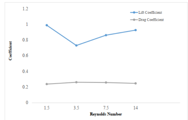
Fig.16 Lift and Drag coefficient variation with spoiler height from rear trunk
