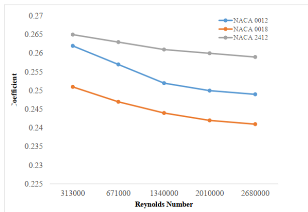
Fig.15 Drag coefficient variation with spoiler at various NACA profile
