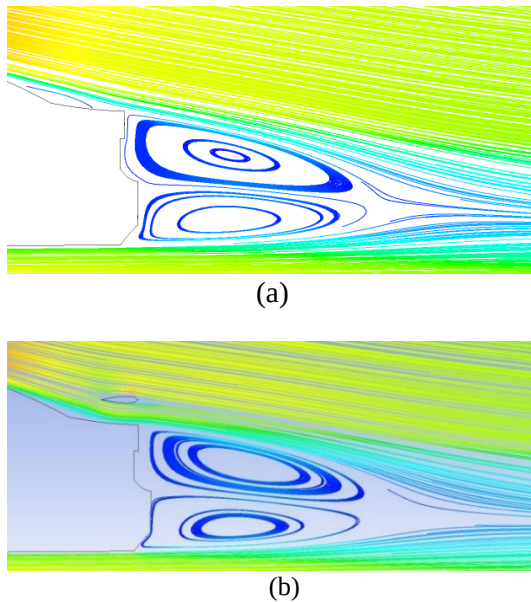
Fig.9 Vortex region at the rear portion of the car (a) Without spoiler (b) With spoiler
