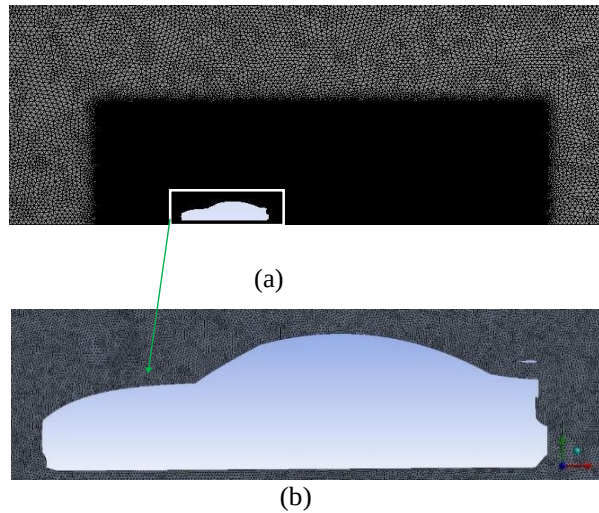
Fig.6 Triangular meshing (a) Meshing all in the domain (b) Meshing near the car body.
