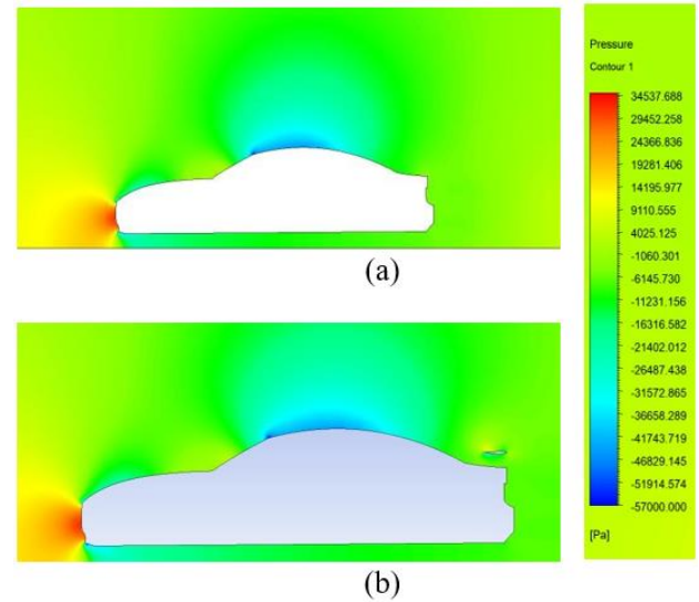
Fig 11 Pressure contour at Reynolds Number 1.34 \times 10^6 (a) Without spoiler (b) with spoiler (NACA 2412)
