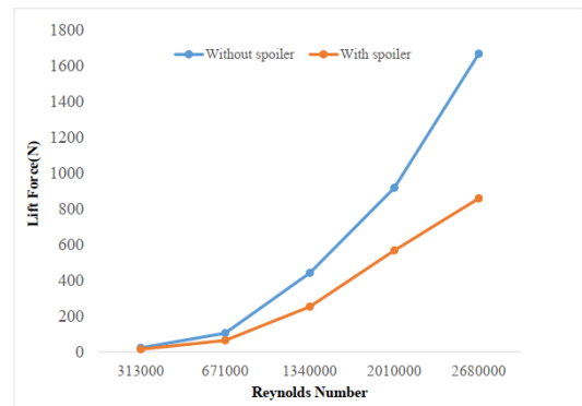
Fig.12 Lift Force variation with Reynolds number
