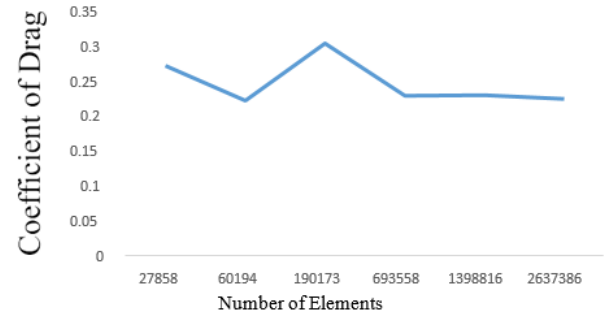
Fig.3 Result of Mesh Dependency Test
