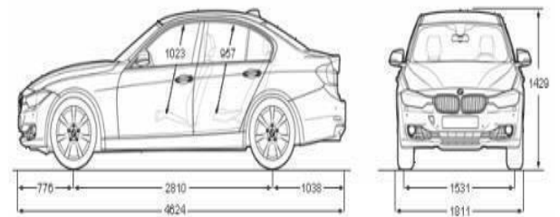
Fig. 4 BMW 316i E Series car model [13]
