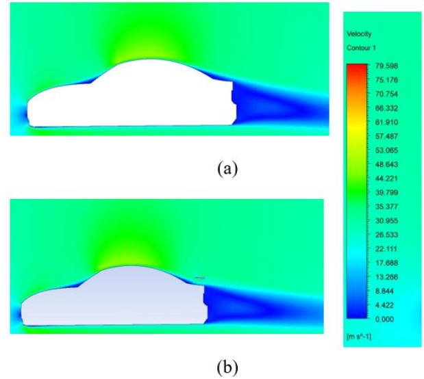
Fig.7 Velocity Contour at Reynolds number Re=2.01 \times 10^6 (a) Without spoiler (b) with spoiler (NACA 0018)
