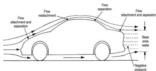
Fig.1 Flow nature over a car body without spoiler [1]
