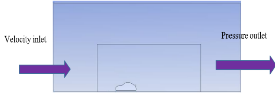
Fig.2 Fluid Domain
